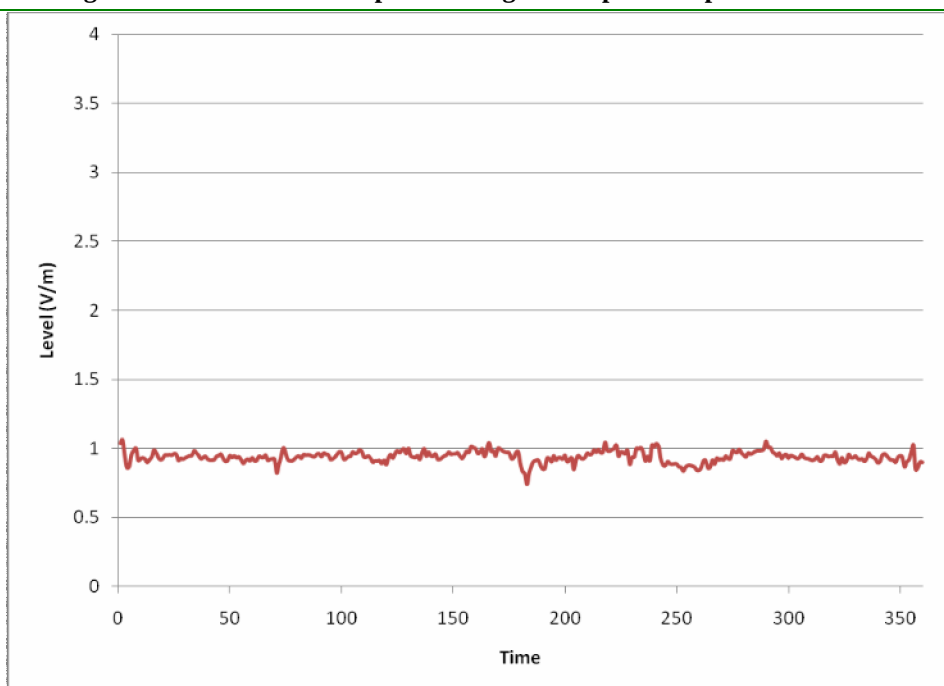
Electric field strengths recorded over 6 min period using 3 GHz probe at point of max NIR:
